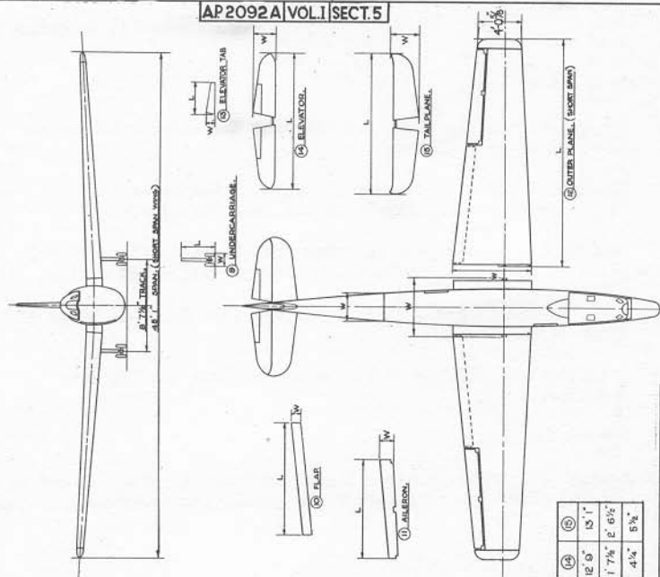
PACKING DIAGRAM
