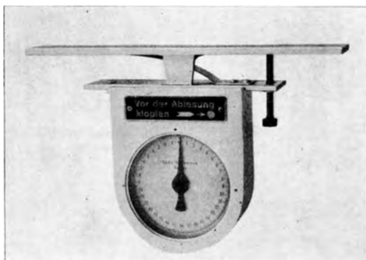
Abb. 378. Anstellwinkelmesser (Wichmann).
