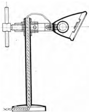
Abb. 289. Soffittenlampe (Ruhstrat).
