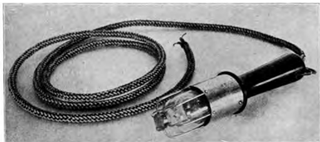
Abb. 285. Stablampe (Ruhstrat).
