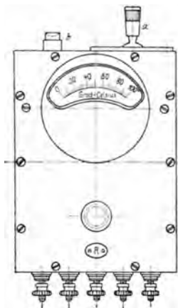
Abb. 80. Fernthermometer (Guggenheimer).
