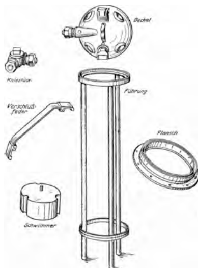
Abb. 55. Benzinuhrflansch Huttenlocher.
