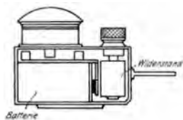
Abb. 282. Handlampe (Ruhstrat).
