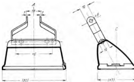
Abb. 287. Soffittenlampe (Ruhstrat).
