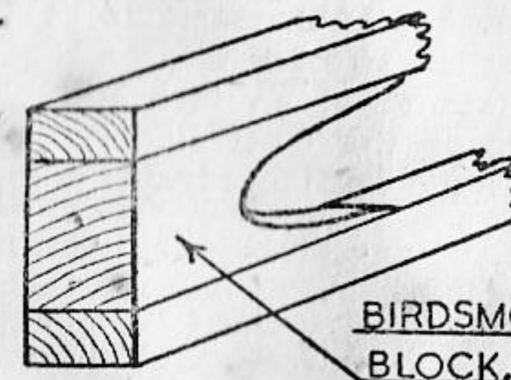
BLOCKED JOINT.
