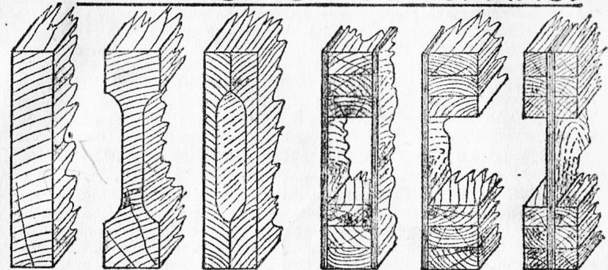
1. SOLID. 2. SPINDLED 3. SPINDLED. 4. BUILT UP BOX SPAR. 5. BUILT UP "U" SPAR. 6. BUILT UP "I" SPAR.
