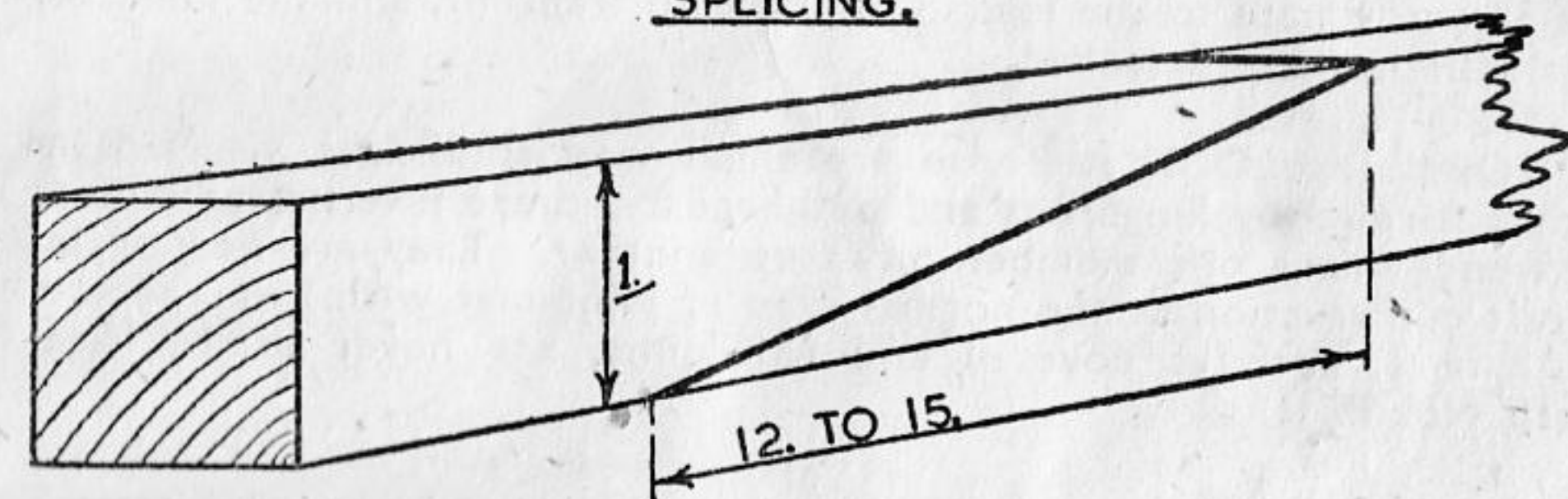
SPLICING.
