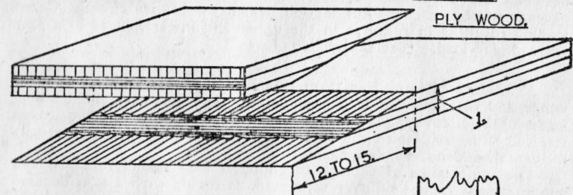
SPLICING.
